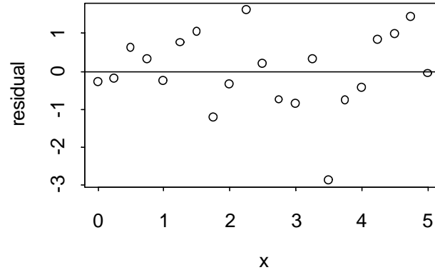
Residual Plot
