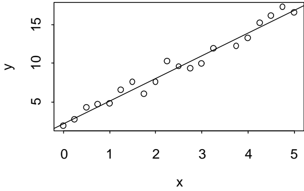
W/W/O Outlier
