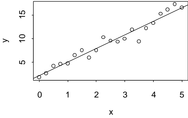
Without Outlier
