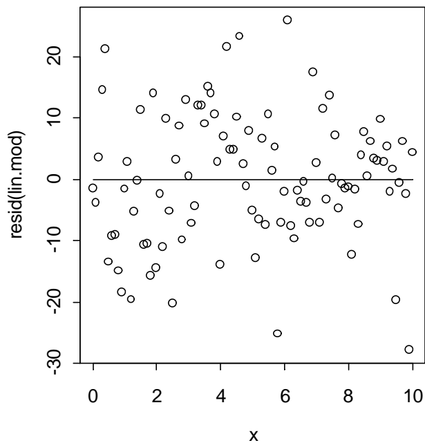
Residual Plot
